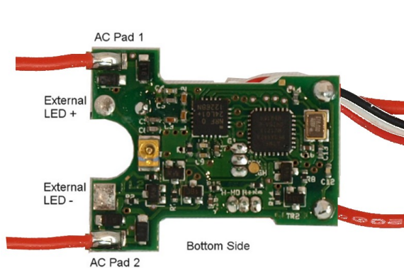
C.SSD ready circuit, bottom side
