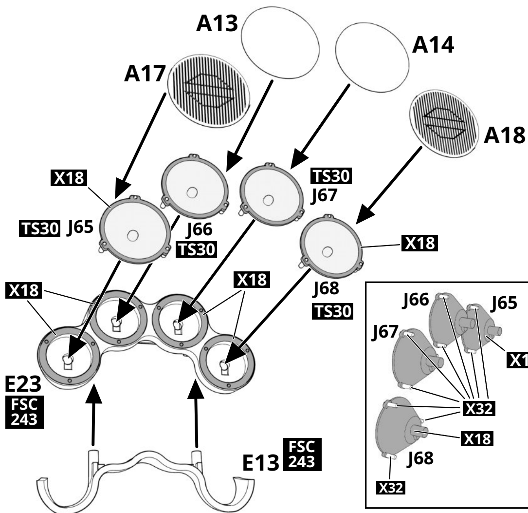
Front Extra Headlights assembly
