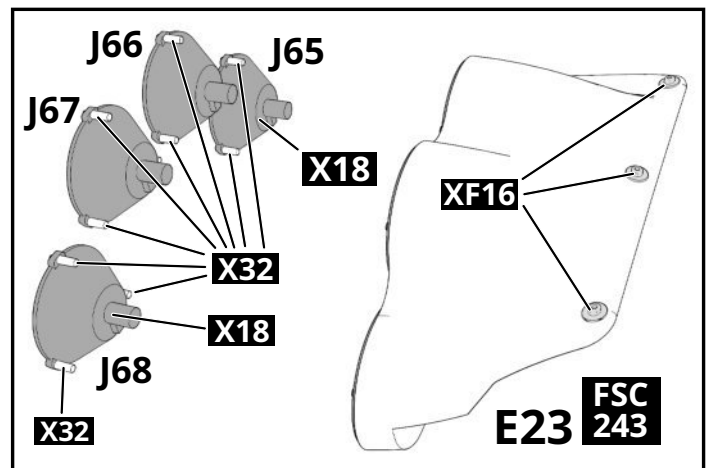
Front Extra Headlights attachment
