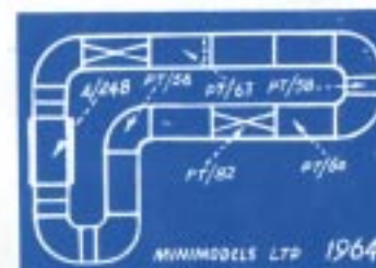
EXTENDED LAYOUT FOR THE '30' SET (see page 2)
